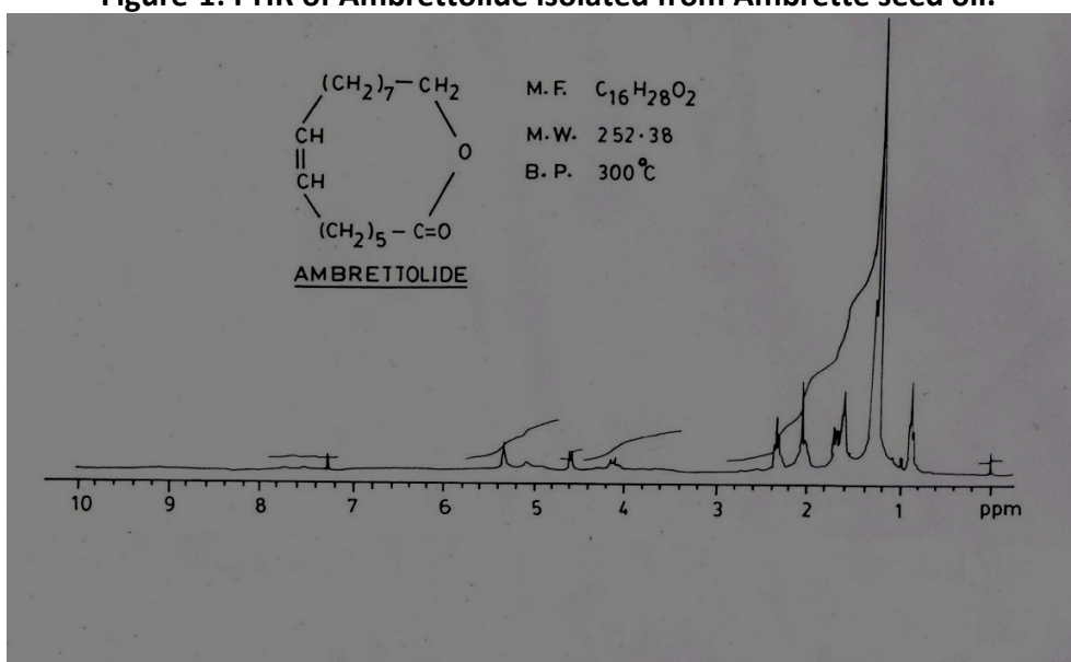
Figure-2: 1 H NMR of Isolated Ambrettolide.
