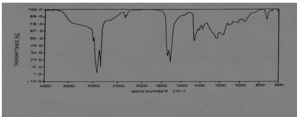
Figure-1: FTIR of Ambrettolide isolated from Ambrette seed oil.
